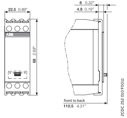
COV.11 - Sealable transparent cover
