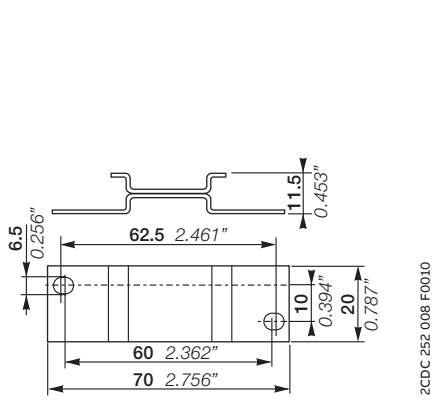
ADP.01 - Adapter for screw mounting
